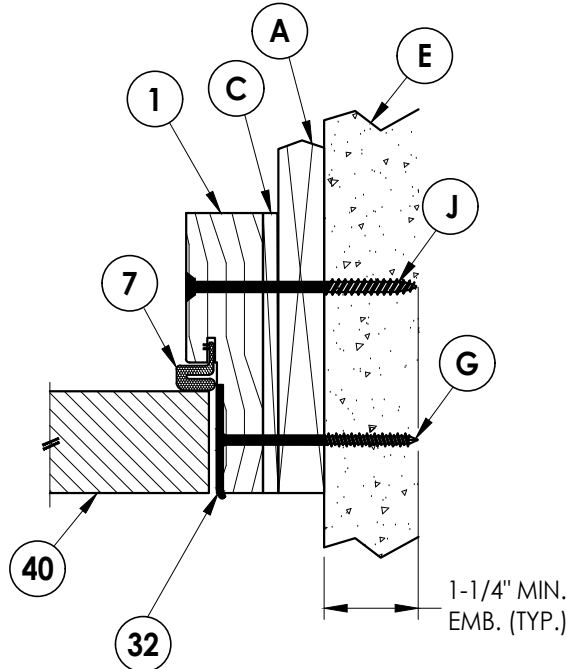
5 6 HORIZONTAL CROSS SECTION Shown w/ 1X Buck Inswing shown (Outswing similar)
