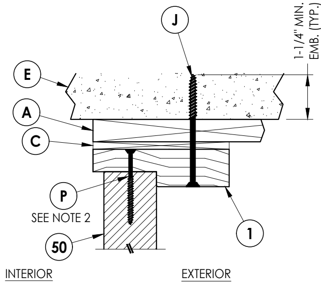
1 6 VERTICAL CROSS SECTION Shown w/ 1X Buck Inswing shown (Outswing similar)
