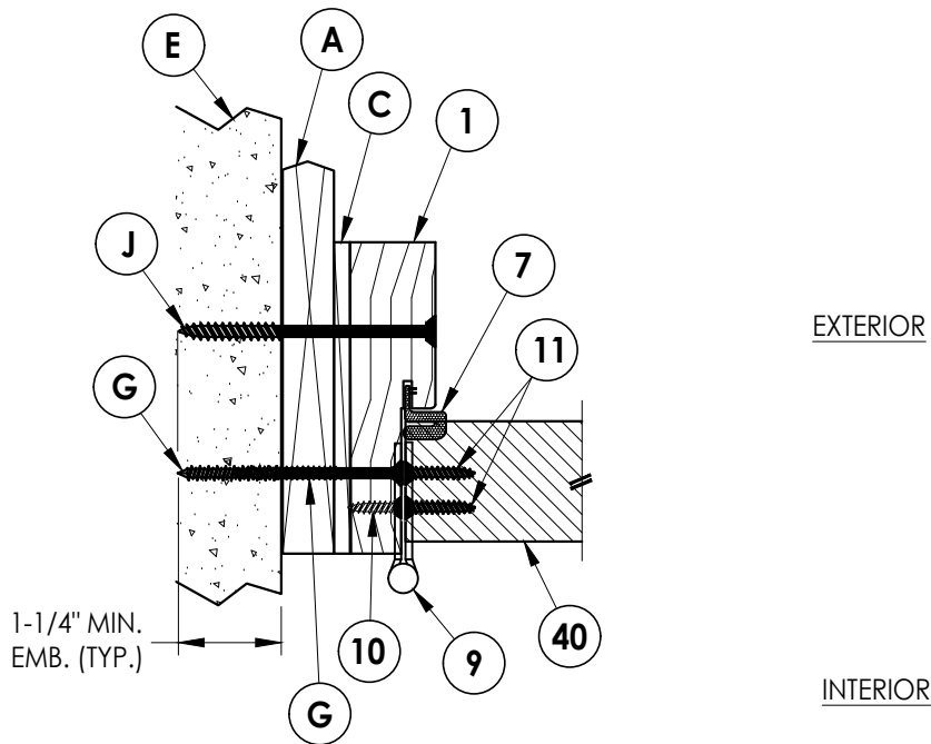
4 6 HORIZONTAL CROSS SECTION Shown w/ 1X Buck Inswing shown (Outswing similar)
