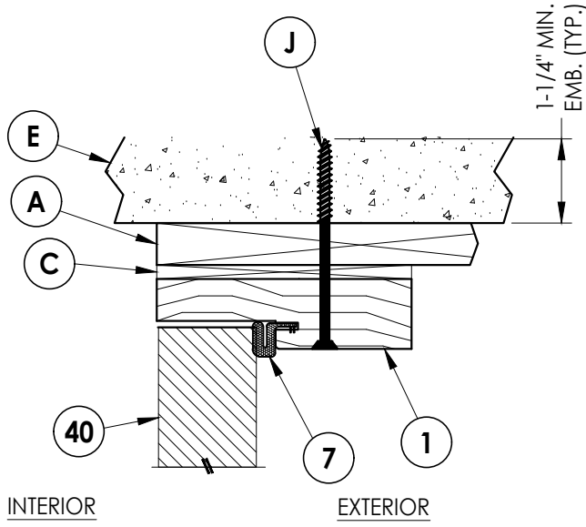
2 6 VERTICAL CROSS SECTION Shown w/ 1X Buck Inswing shown (Outswing similar)
