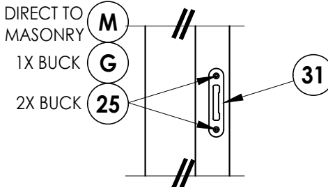
MULTIPOINT TONGUE STRIKE DETAIL
