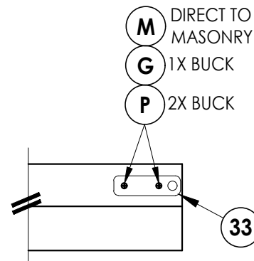
SHOOTBOLT STRIKE @ HEAD 1" X 3-3/8" STEEL PLATE (0.10" THICK)
