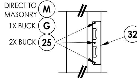
MULTIPOINT LATCH & DEADBOLT STRIKE DETAIL
