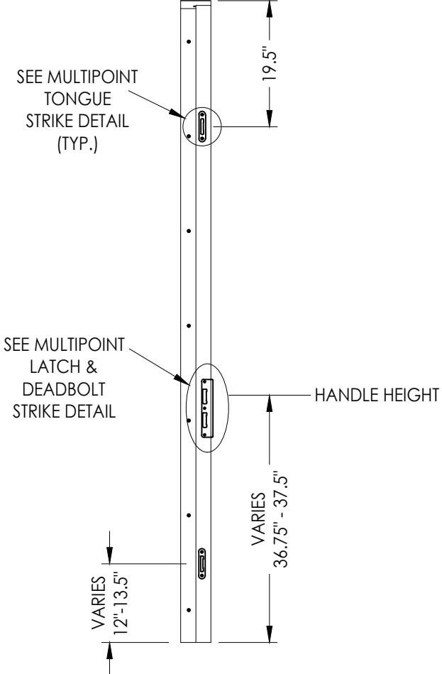
STRIKE JAMB HOPPE MULTIPOINT LOCK
