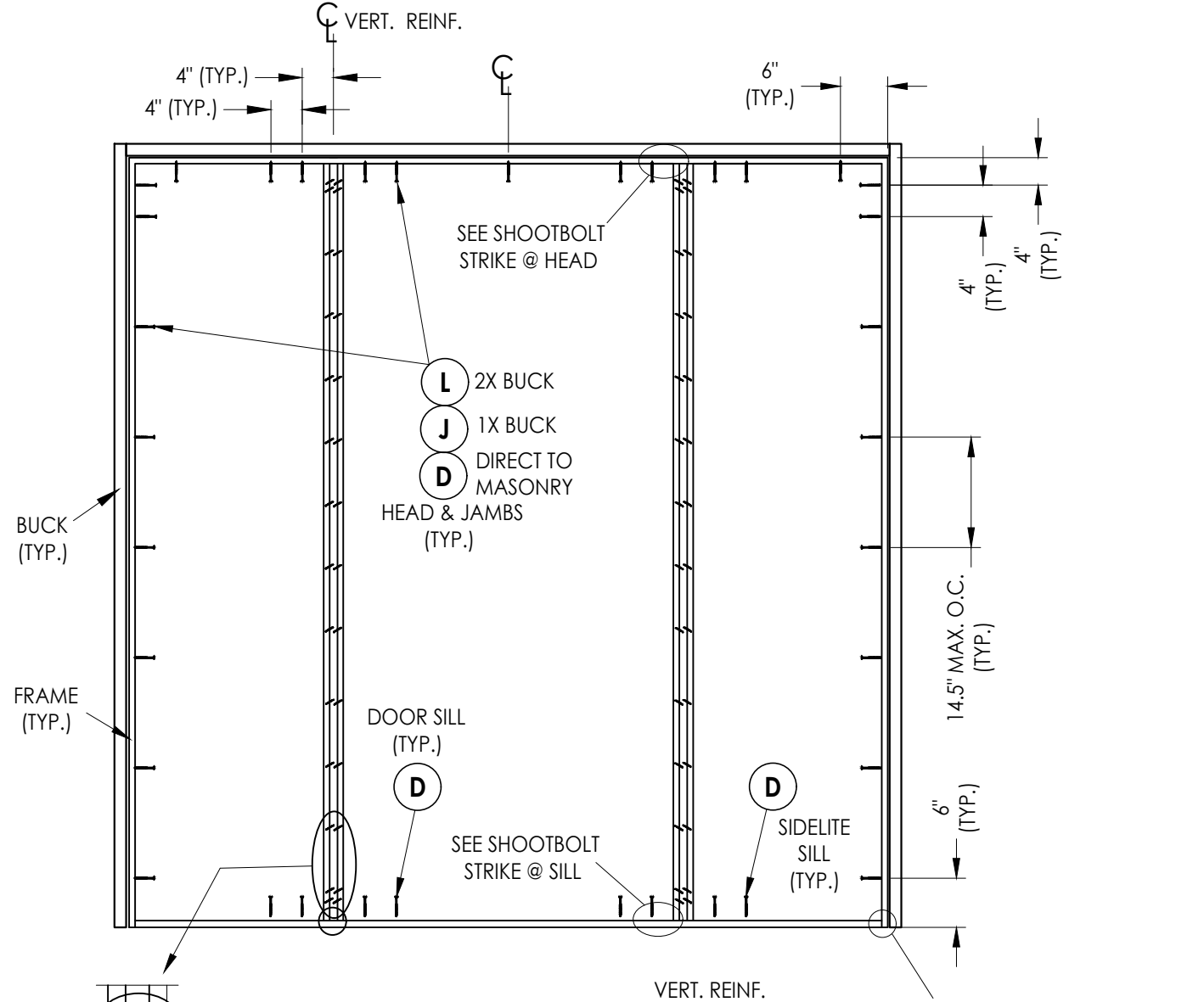
FRAME ANCHORING OXO
