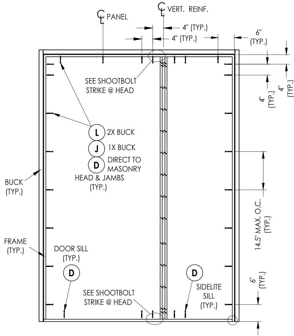
FRAME ANCHORING XO/OX
